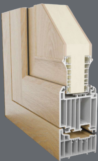
DOUBLE RAISED & FIELDED PANEL 44mm only
